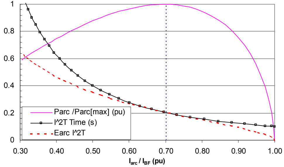
Figure A.11: Plot of arc power, trip time and arc energy released as function of arc current. All values in the plot are normalized: P_{\text{arc}} is in per unit of maximum arc energy ( 0.5 * \text{MVA}_{\text{BF}} ); trip time for inverse square curve ( I^2T ) is 0.1 seconds for I_{\text{arc}} = I_{\text{BF}} ; E_{\text{arc}} is normalized P_{\text{arc}} times arcing time.
