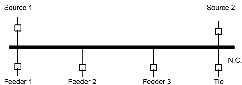
Figure 5.2: Dual Sources
