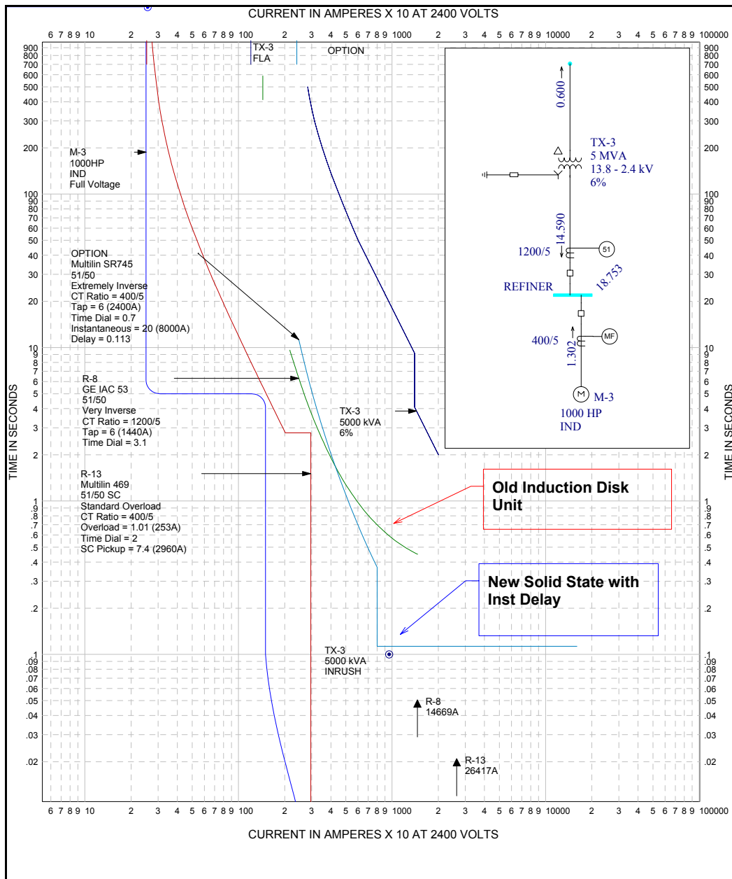
Figure B.10: Relay trip time compared with solid state device.
