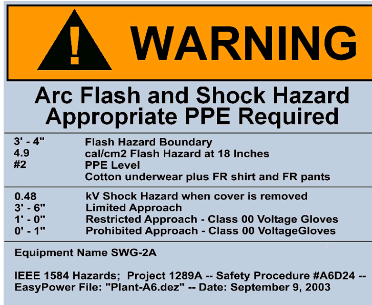
Figure B.14: Warning label that can be printed directly from EasyPower ArcFlash program.
