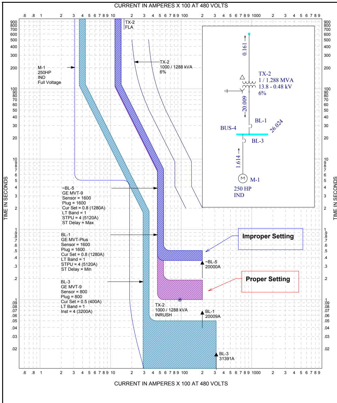
Figure B.8: Typical example of improper trip delay setting.
