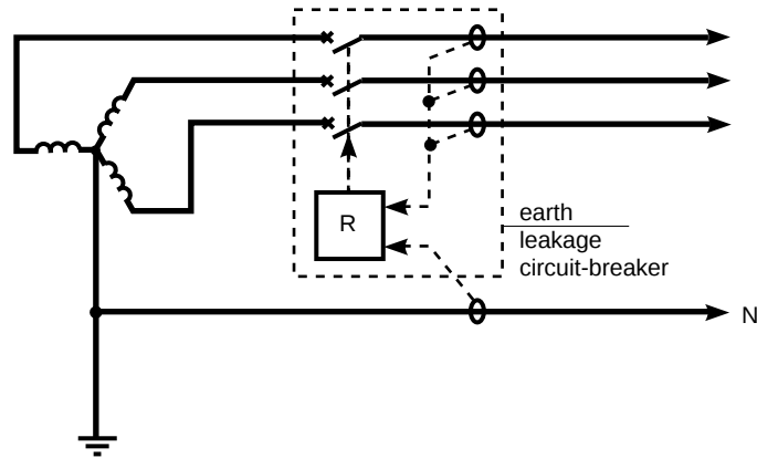
fig. 14: residual sensing.
