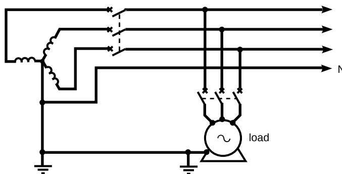
fig. 13: TN-S earthing system in the USA.
