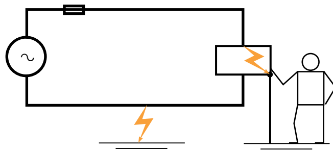
fig. 2: the emergence of the unearthed neutral.
