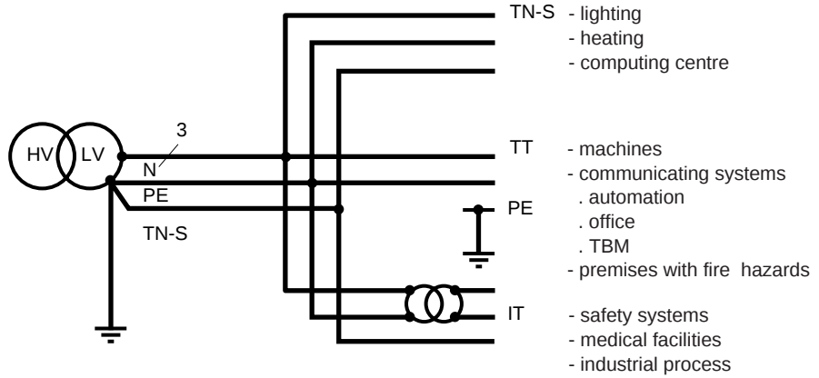
fig. 24: several earthing system included in the same LV installation.
