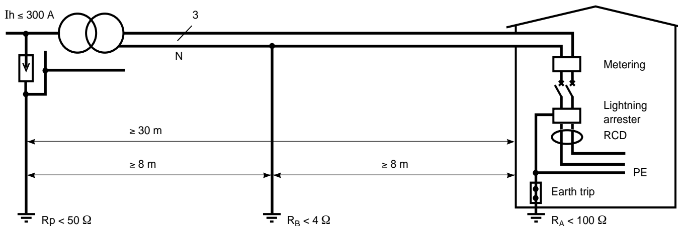
Fig. 20 : rural overhead public distribution in France.
