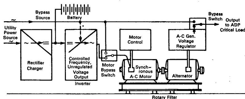
Figure 54. Uninterruptible synchronous motor-generator set: This uses a solid-state ac/dc rectifier-charger and dc/ac inverter to drive the m-g set for constant frequency and voltage output. The m-g set acts as a "rotary filter" with rotational energy storage to regulate and smooth voltage wave shape, and to handle momentary overloads. An optional motor bypass switch allows the m-g set to be used as a line filter and regulator while solid state equipment or batteries are being serviced.
