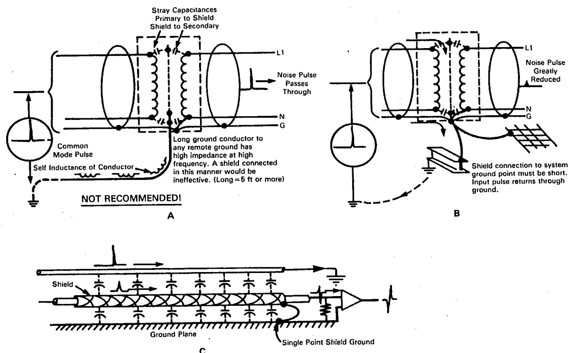
Figure 16. Grounding of shields: (a) A long shield return path makes an interwinding shield ineffective; (b) A short shield path to the system ground reference reduces pulse noise at the output; (c) Where a single point ground on one end of a shield may be ineffective above 1-10 MHz, multipoint grounding of an outer shield may be required.
