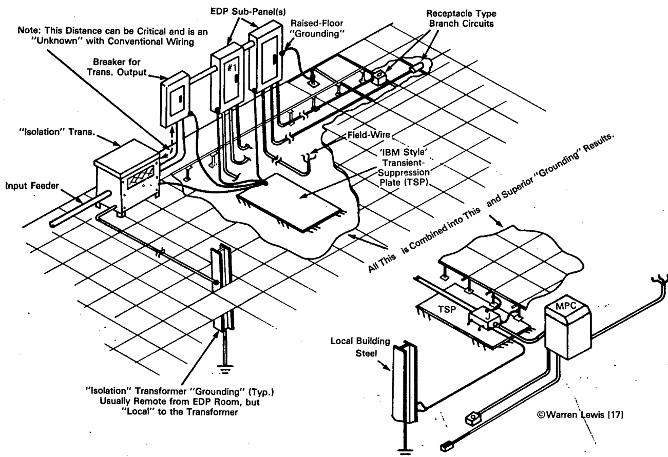
Figure 36. Transient Suppression Plate (TSP) installation details.
