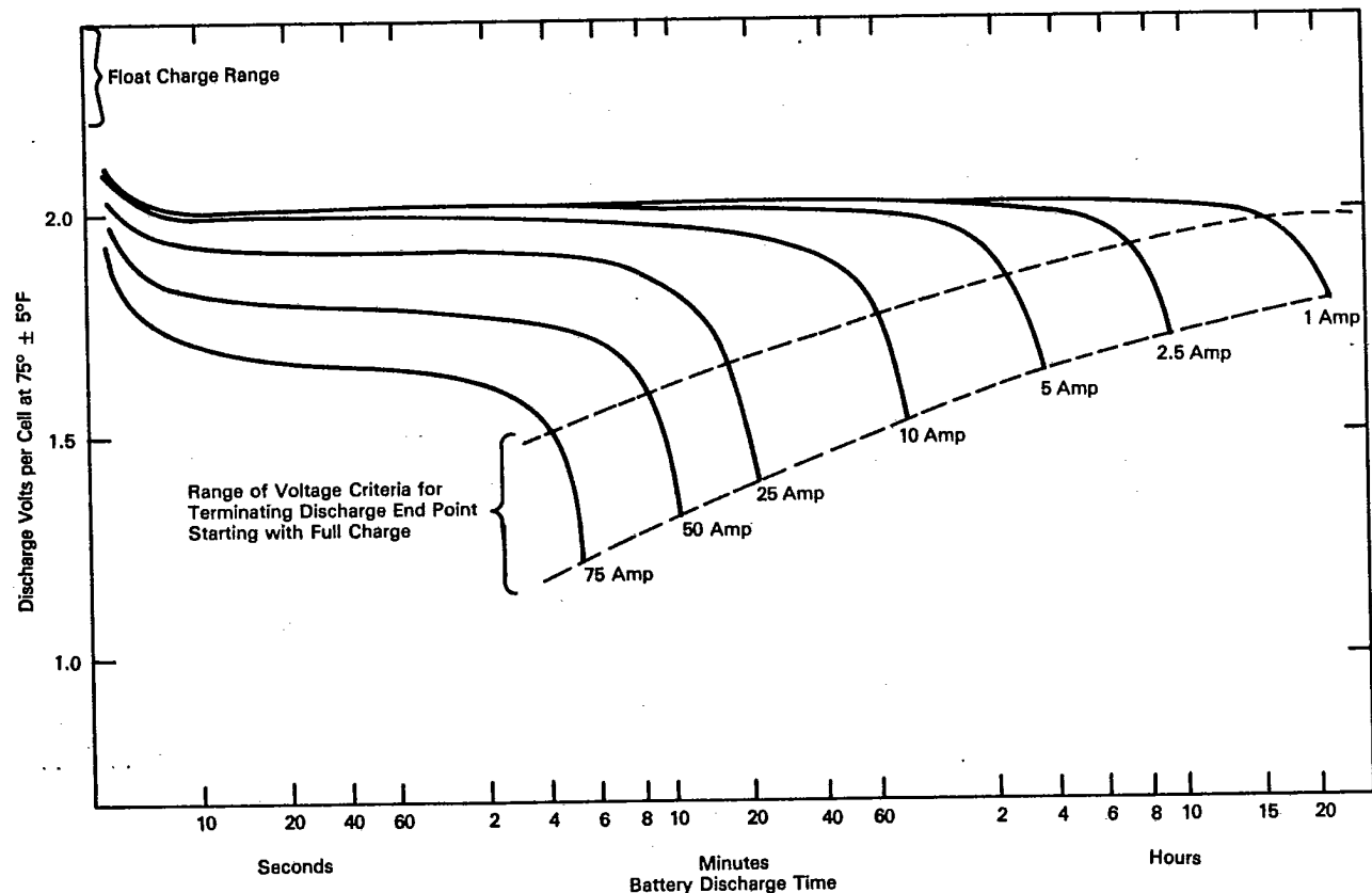
Figure 60. Typical battery discharge characteristics.
