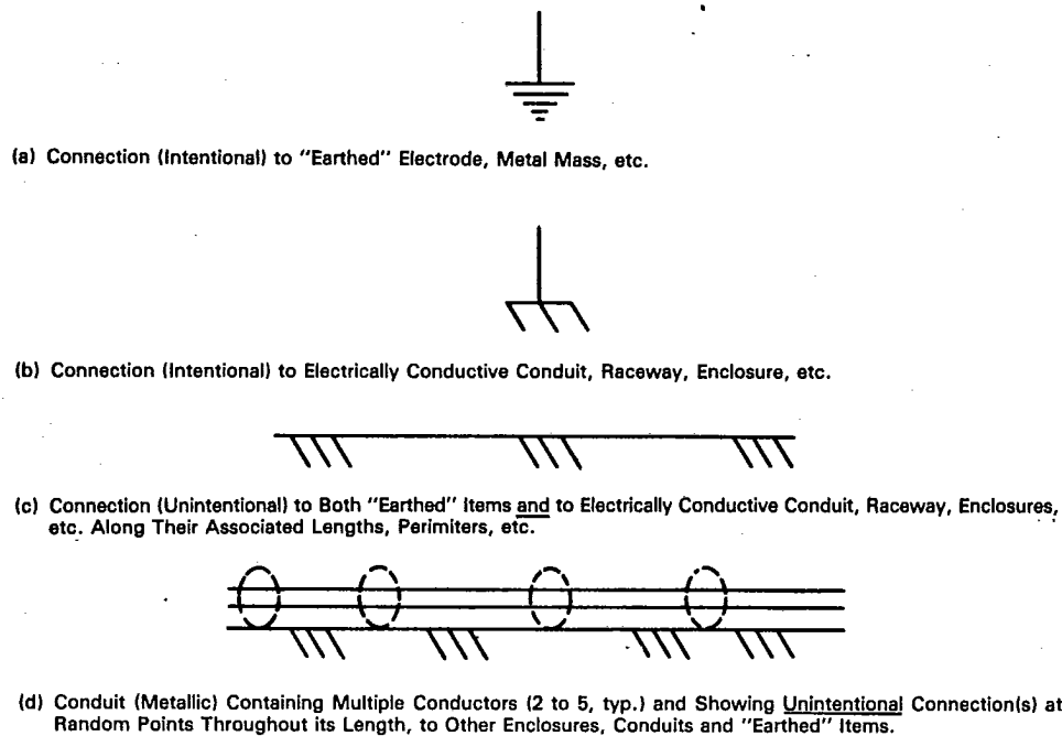
Figure 35. Symbols which appear in schematic and pictorial diagrams.
