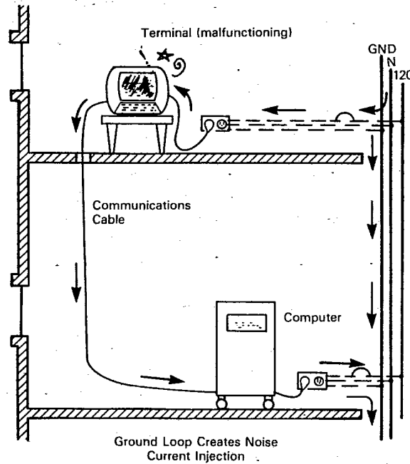
Figure 25. An unwanted ground loop is created by grounding two ADP units to separated points on a bus duct ground conductor. The resulting noise current in the data cable creates errors and malfunctions.
