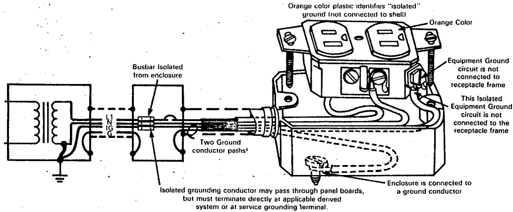
Figure 22. Isolated ground receptacles: When installed per National Electric Code Article 250-74, Exception 4, at least two ground conductor paths are required; one for the receptacle ground pin and the other for the receptacle enclosure.
