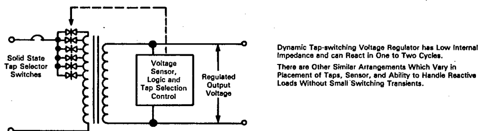
Figure 45. Line voltage adjusters: Dynamic tap-selecting electronic switch changes taps to keep output voltage within an acceptable range. It has the high efficiency, low internal impedance and overload capability of a good transformer. Some units are supplemented with surge limiters and filters.
