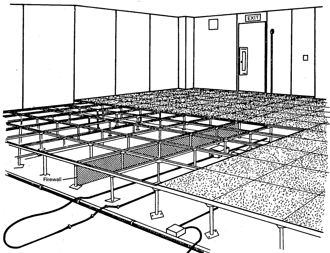
Raised Floor Supporting Structure as a Signal Reference Grid
