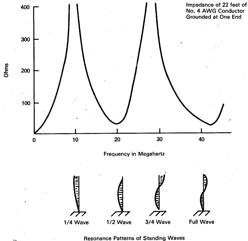
Figure 29. Resonance characteristics of conductors: These are typical of grounding conductors used in ADP systems, although lengths and natural frequencies will vary.
